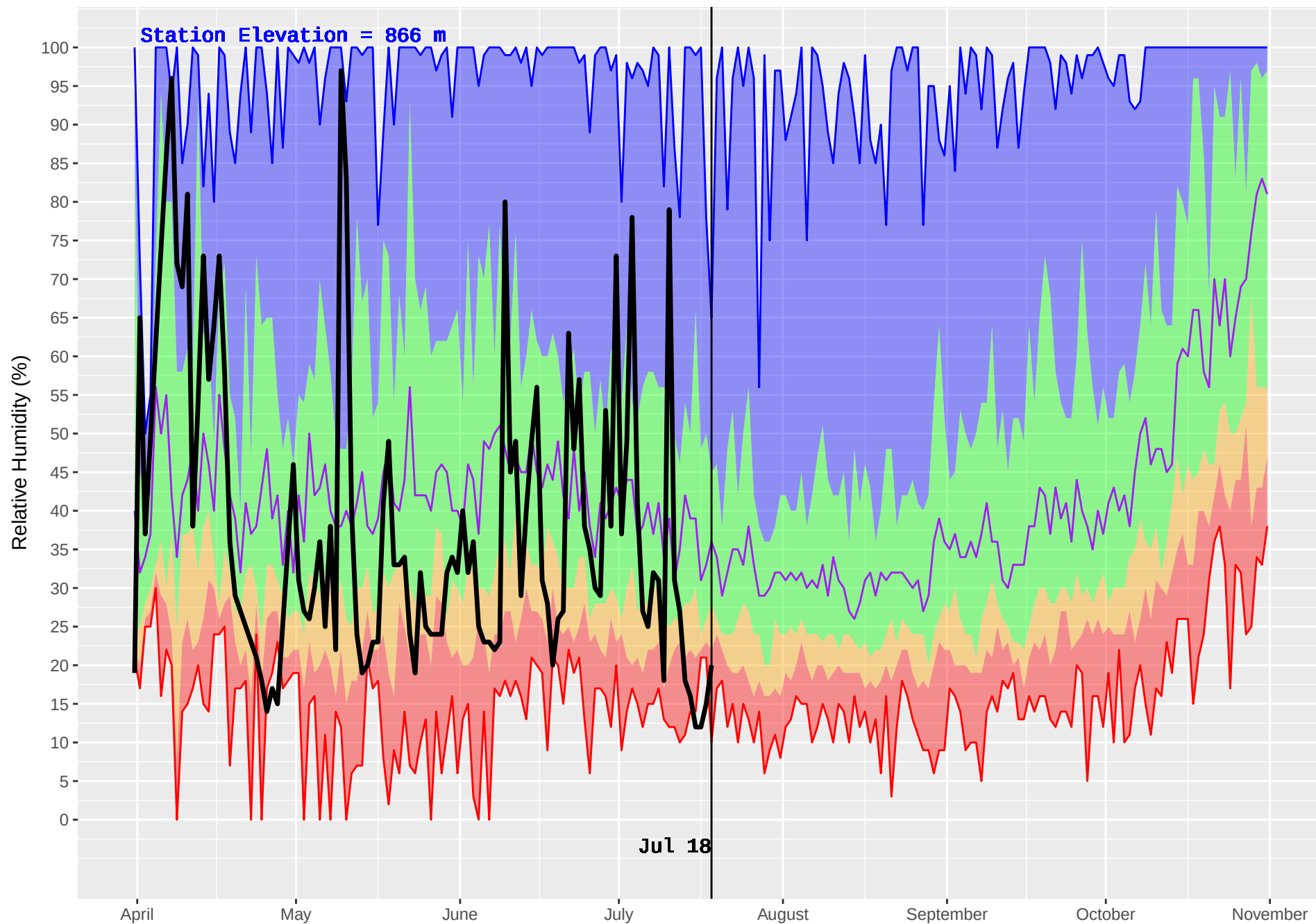
NICOLL (393) : Historical (1981–2016) and Current (2018) Daily Relative Humidity
