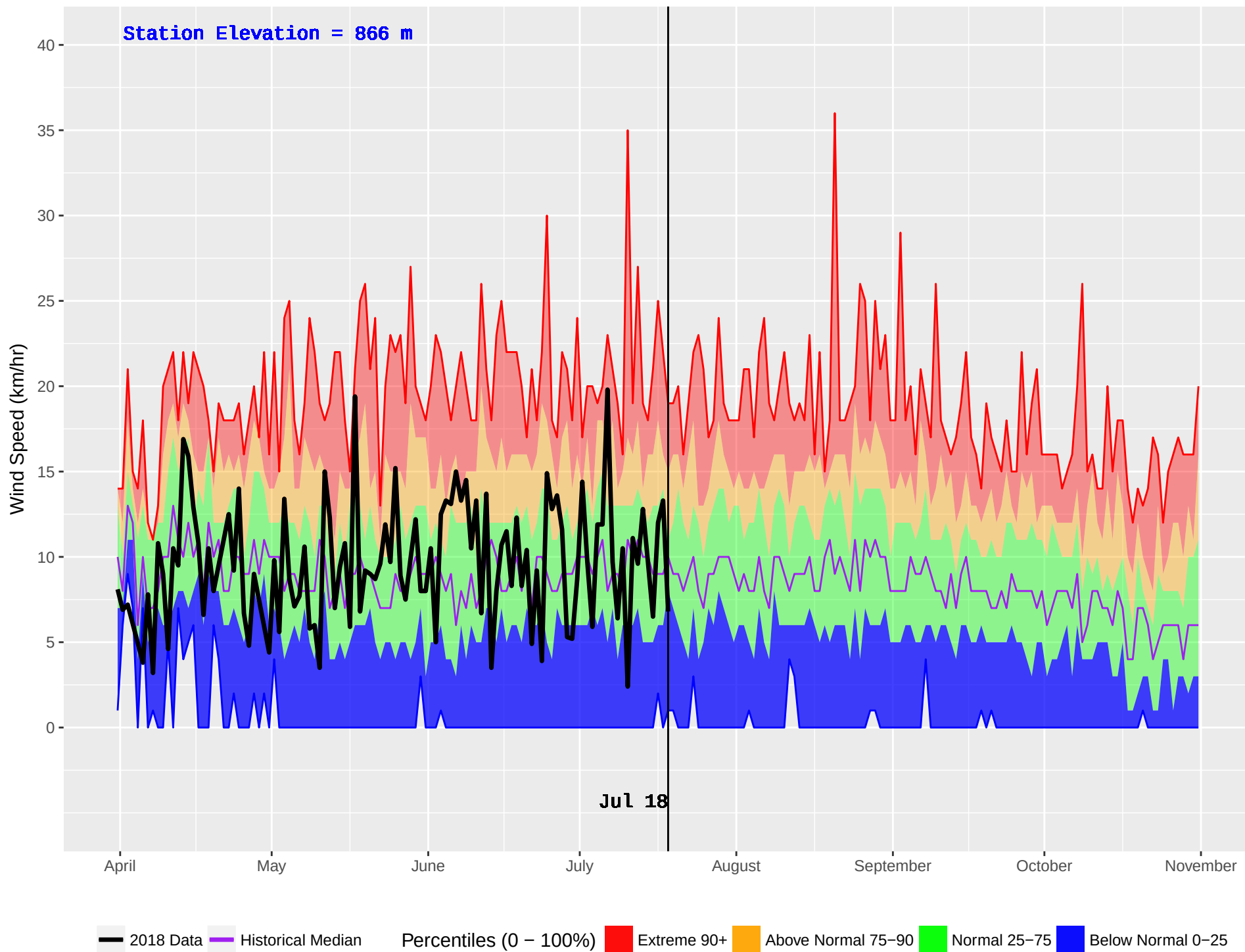
NICOLL (393) : Historical (1981–2016) and Current (2018) Daily Wind Speed
