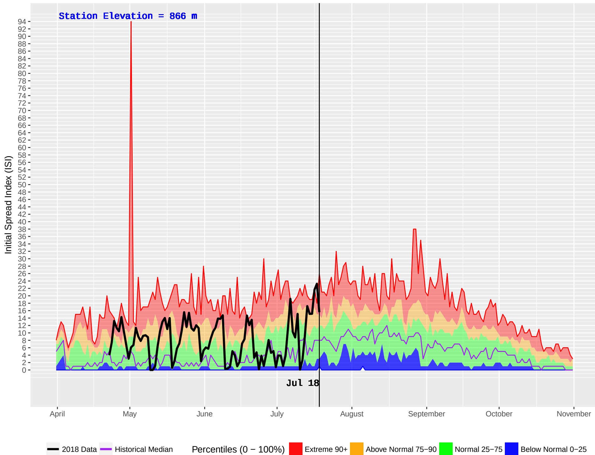
NICOLL (393) : Historical (1981–2016) and Current (2018) Daily Initial Spread Index (ISI)
