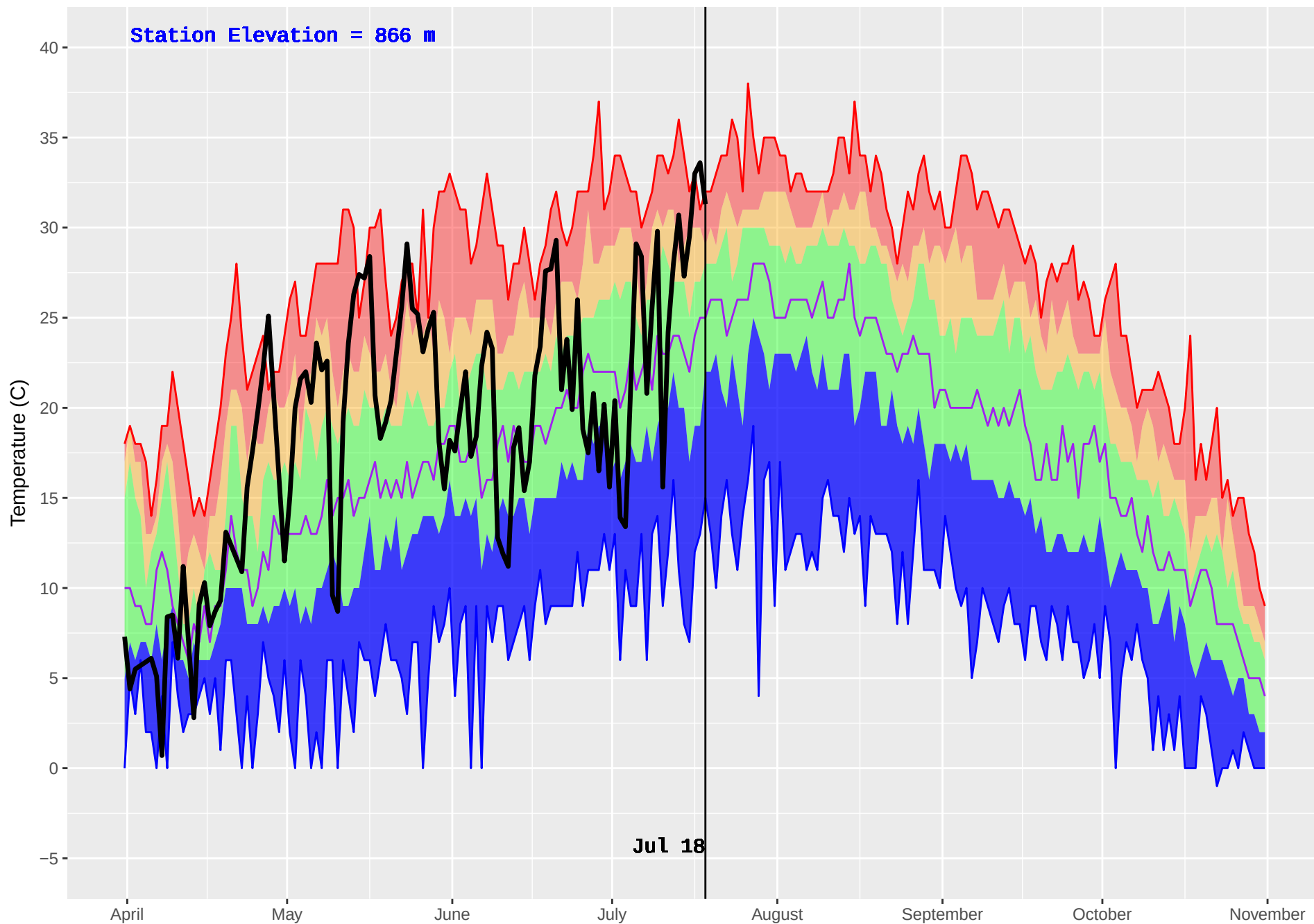
NICOLL (393) : Historical (1981–2016) and Current (2018) Daily Temperature
