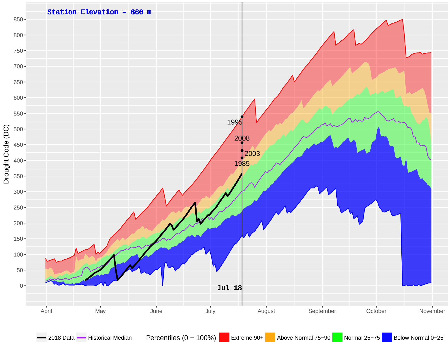
NICOLL (393) : Historical (1981–2016) and Current (2018) Daily Drought Code (DC)
